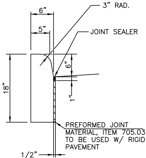
CURB TYPE 6
