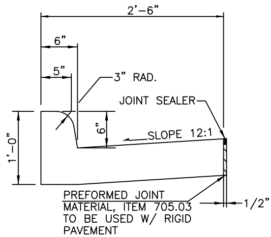
CURB TYPE 2
